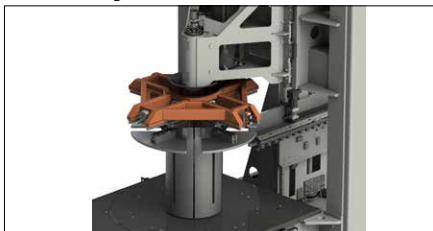
Abb. 6 Ringwickelstation
