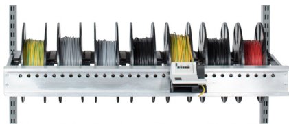
Fig. 14 Cable guiding rail
